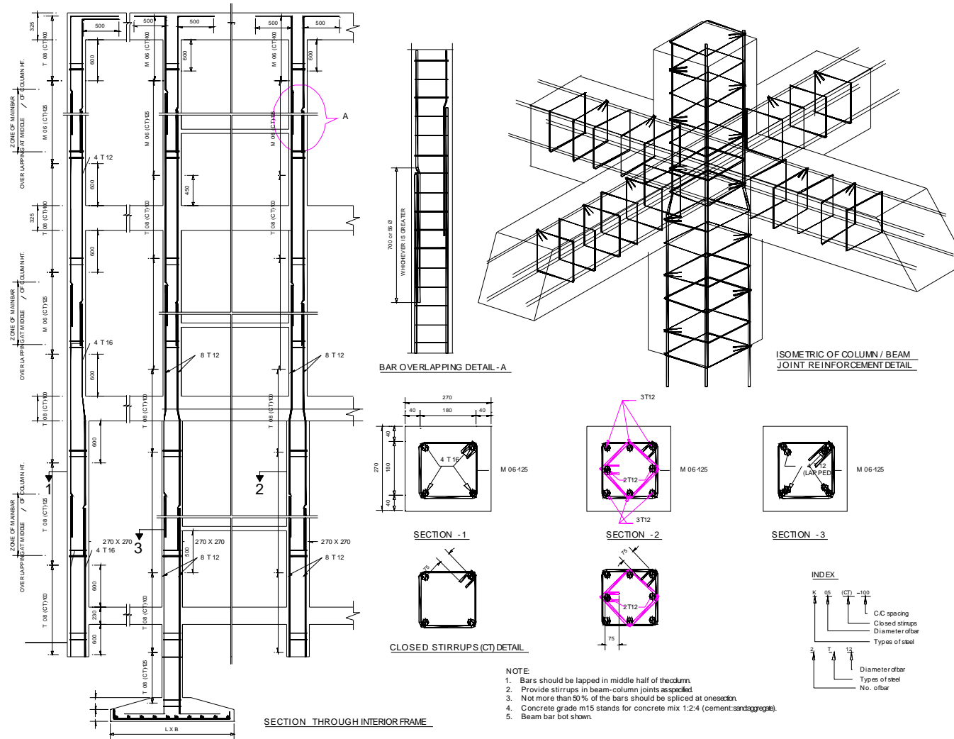
Figure 7.3 : Column Detail
