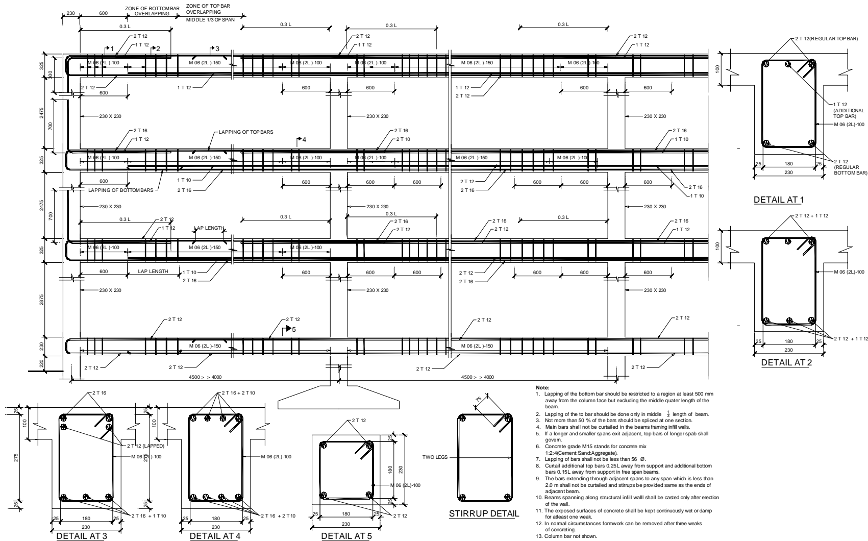
Figure 7.2 : Beam Details
