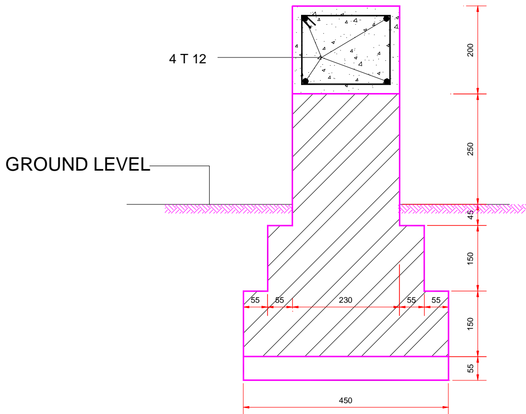
Figure 7.5 : Toe Wall Details
