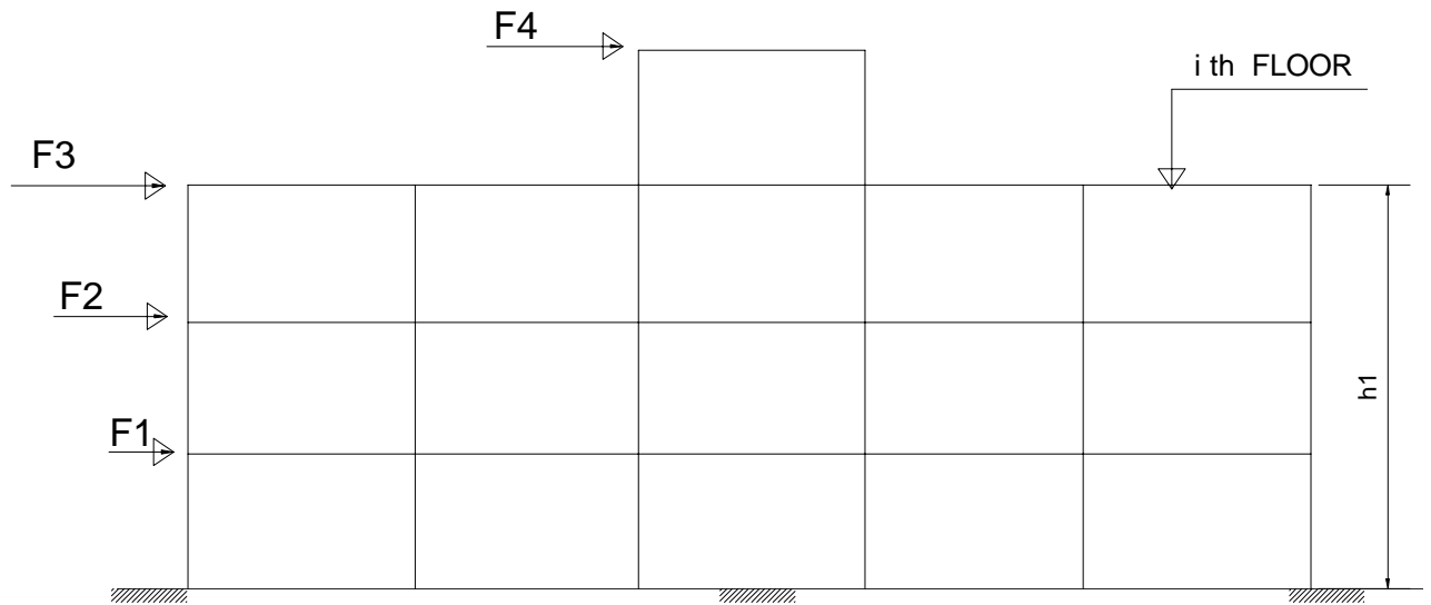
Figure 6.1 : Floor Level Lateral Forces
