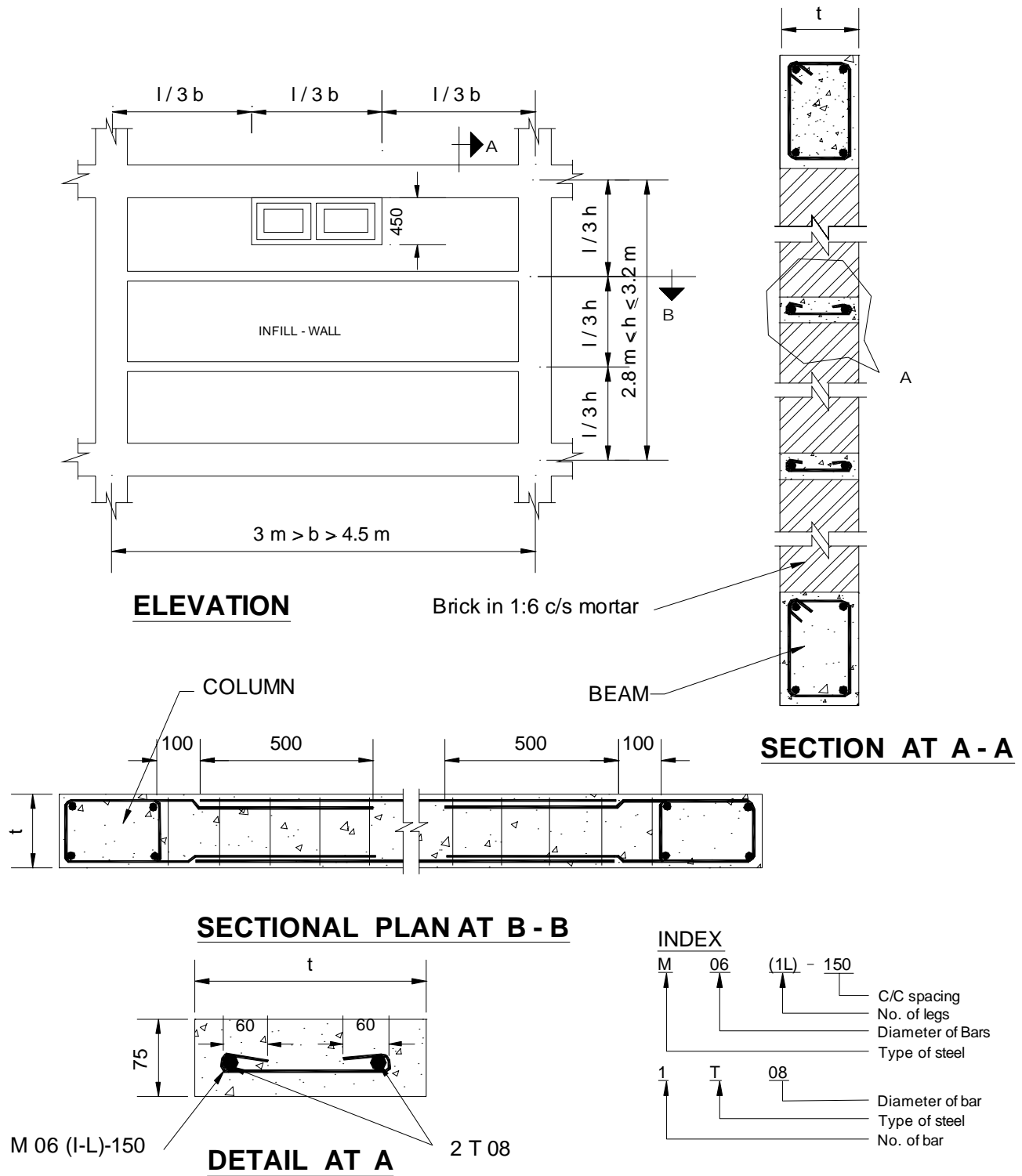
Figure 8.1 : Tie-Band Detail of Solid Walls
