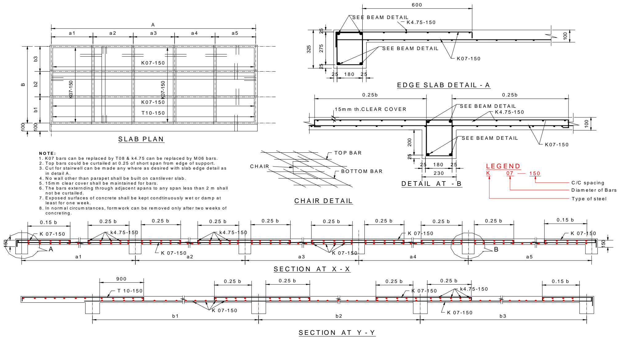
Figure 7.1 : Slab Reinforcement Details
