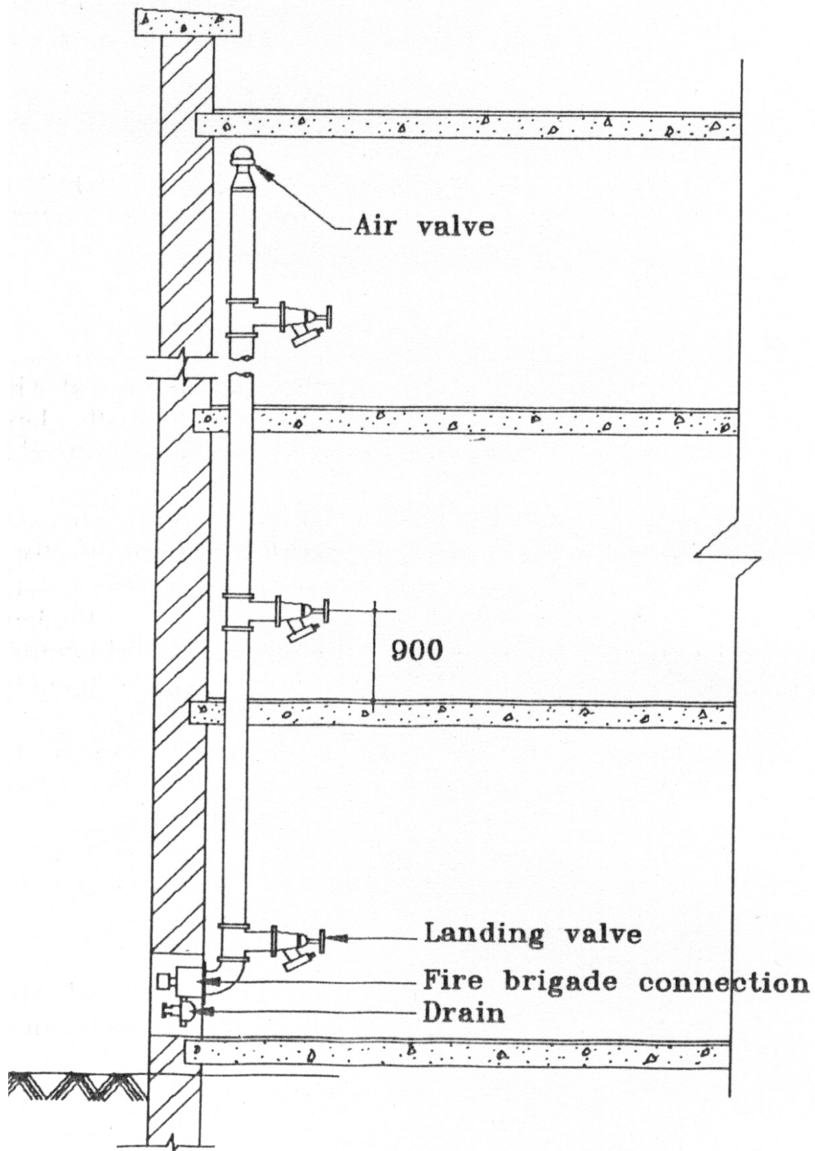
Dry Riser/Fire Fighting Installation Illustration A3
