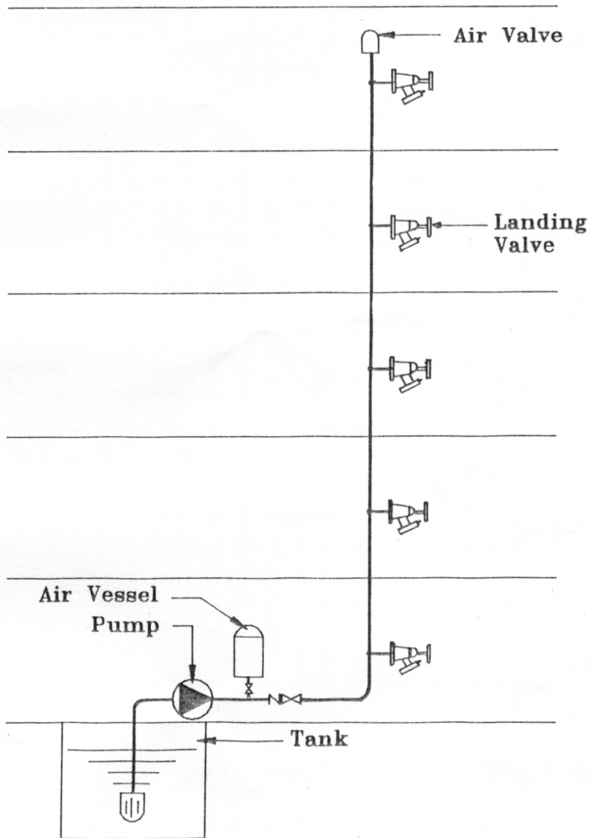
Wet Riser/Fire Fighting Installation Illustration A4
